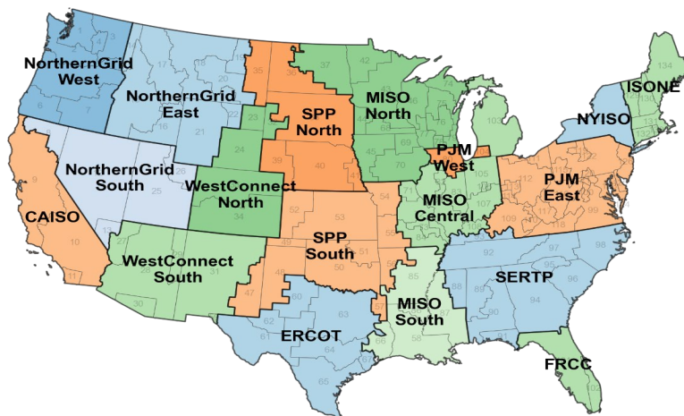
Figure C2 - Geographic Regions for Projected Electricity Emissions Factors for the Contiguous United States. Source: Cambium 2024, U.S. National Laboratory of the Rockies
